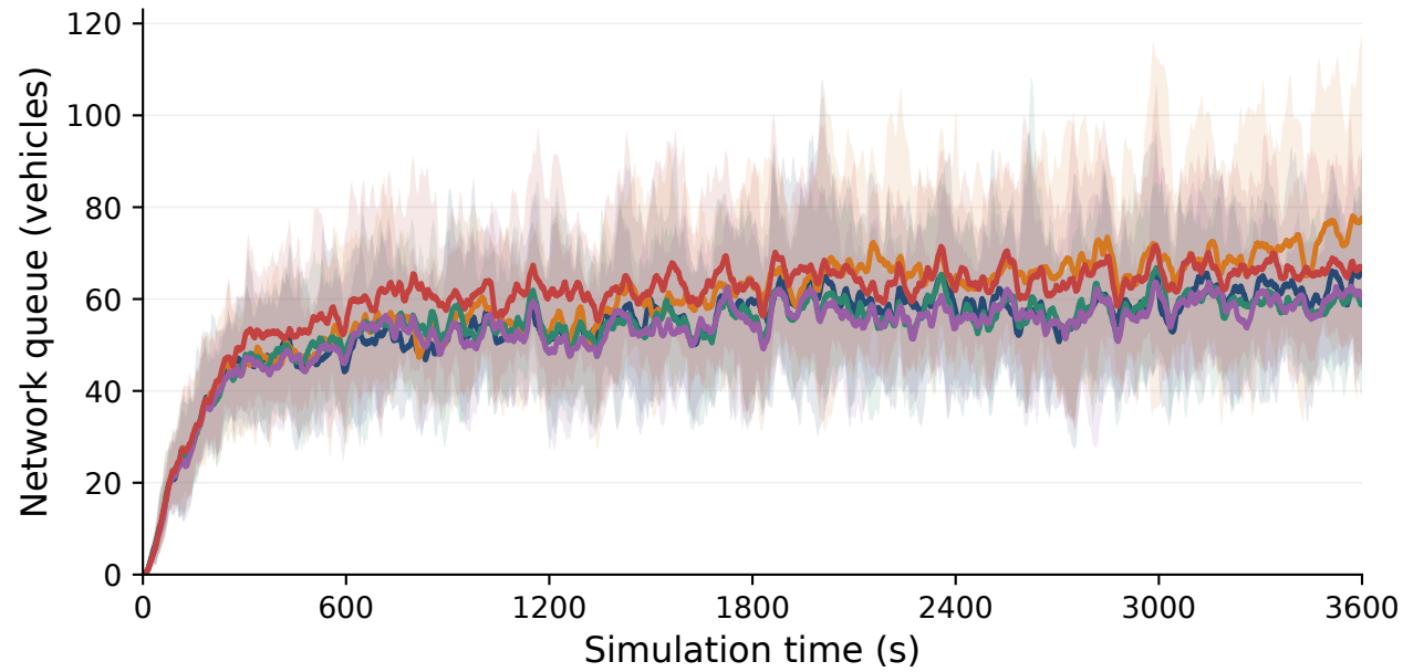
IA2C
